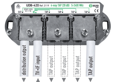
Connection for a distribution network
