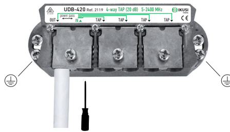
Closing the flange cover by means of the screw
