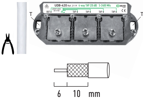
Wall fixing (T) Coaxial cable stripping
